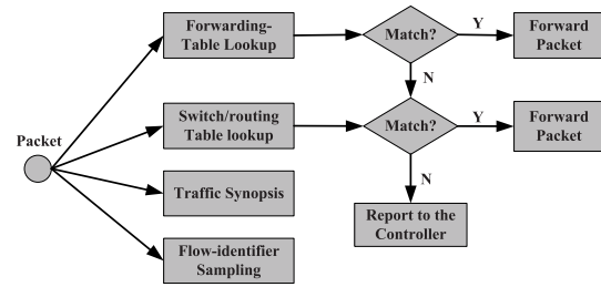
Fig. 3. Illustration of real-time packet processing.
